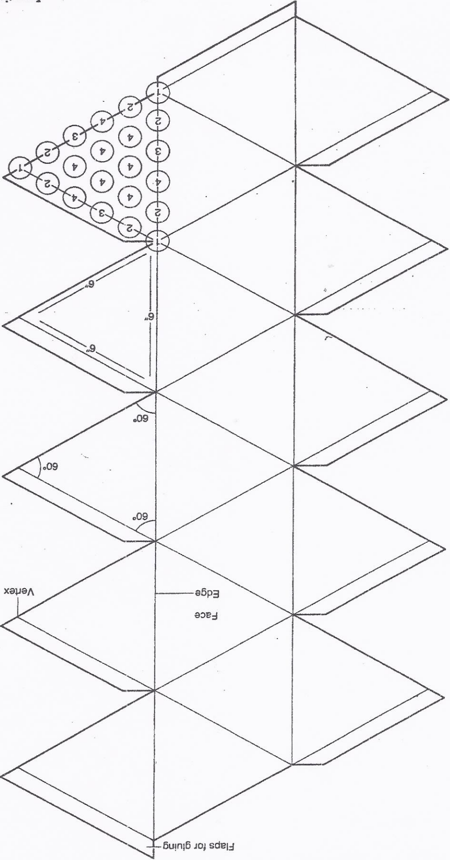
Template for an Icosahedron
