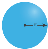
SPHERE V = \frac{4}{3} \pi r^3
