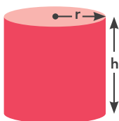
CYLINDER V = \pi r^2 h
