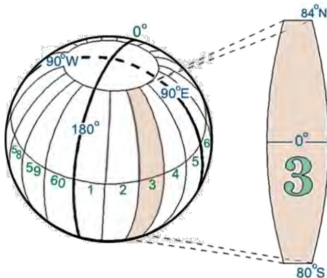
Grid Zones of the UTM Grid System
