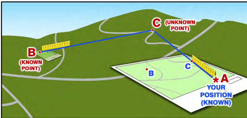
Using Intersection: The Straightedge Method
