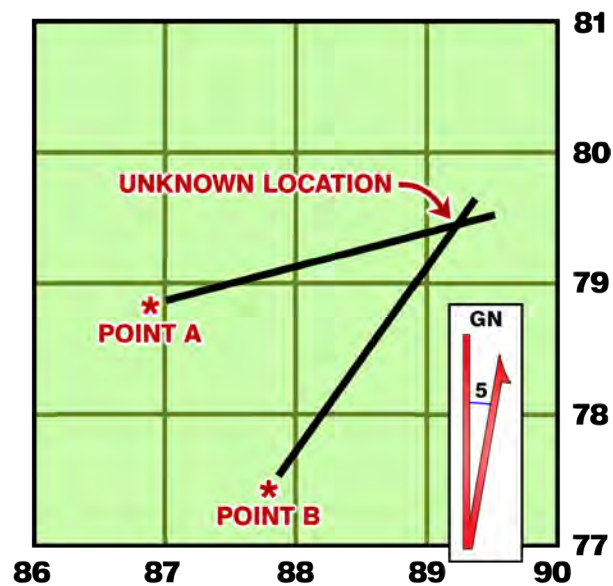
Using Map and Compass: The Intersection Method
