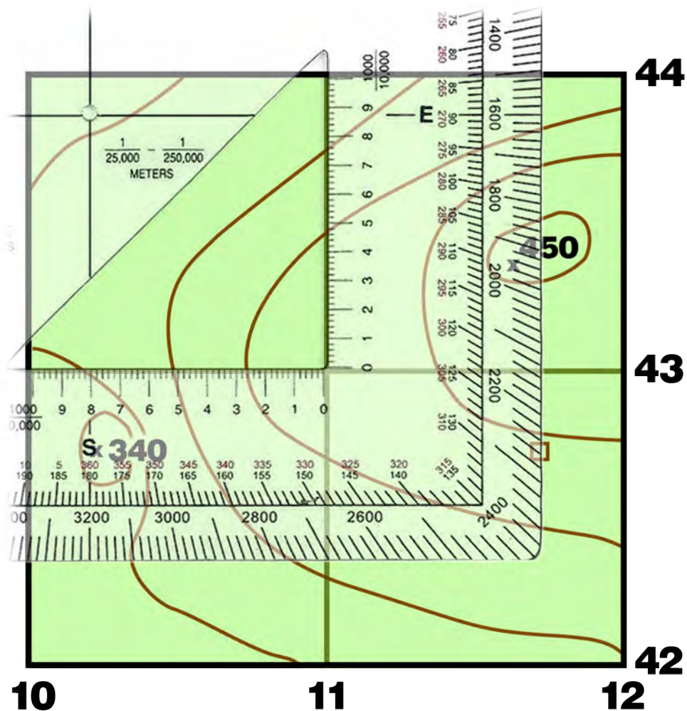
Placing the Coordinate Scale
