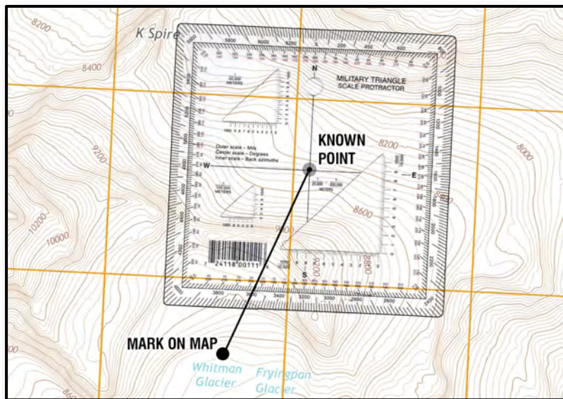
Using a Protractor to Plot a Grid Azimuth
