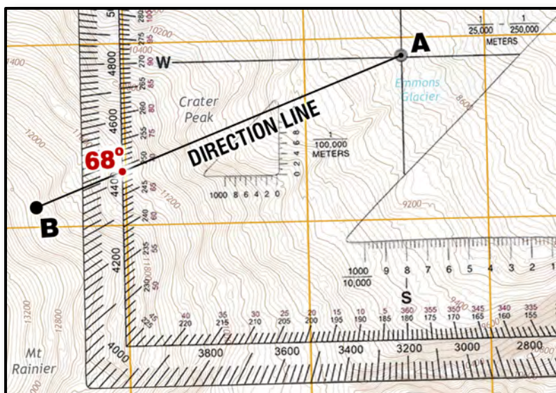
Using a Protractor to Measure a Grid Azimuth
