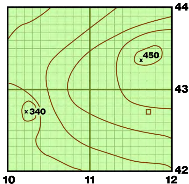
Determining an Eight-Digit Grid Coordinate
