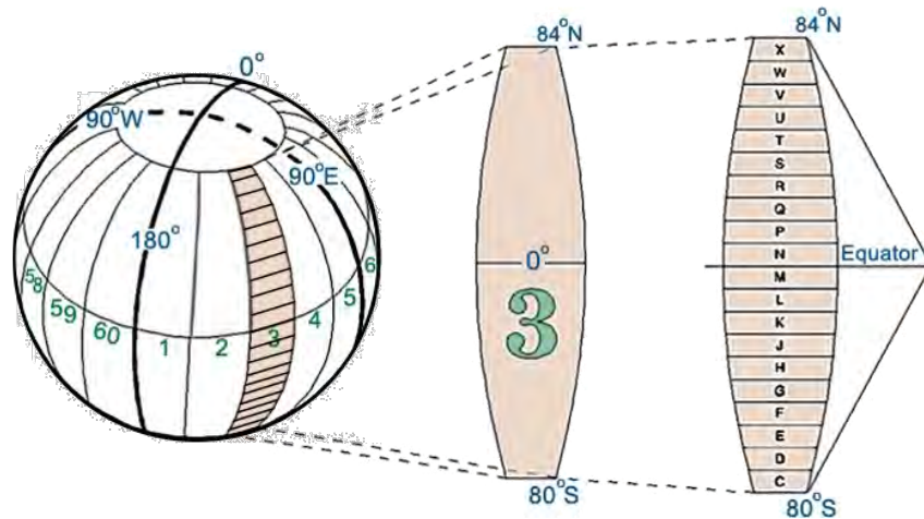
Grid Segments of the UTM Grid System
