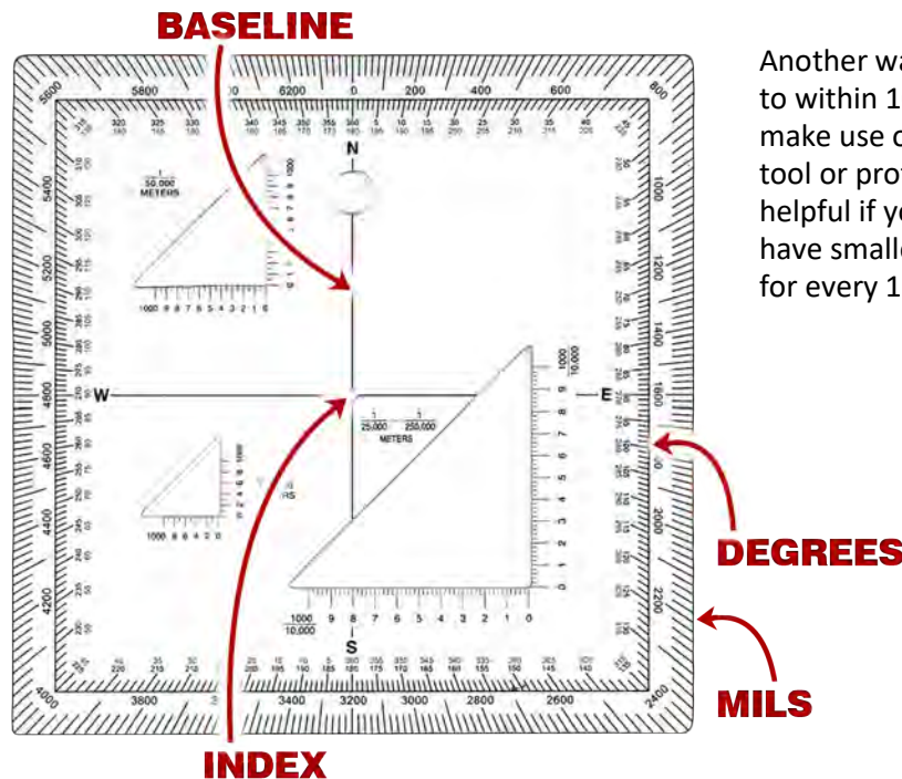
The Army Coordinate Scale
