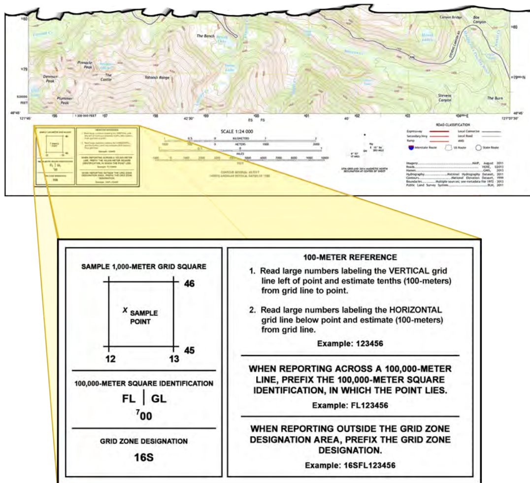
A Grid Reference Box
