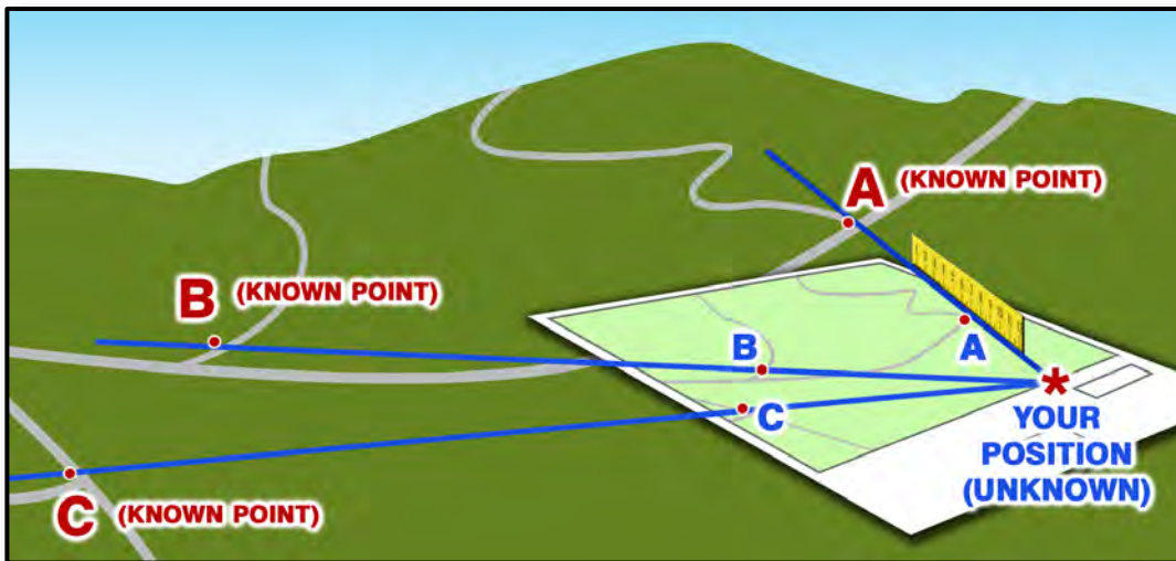
Using Resection: The Straightedge Method
